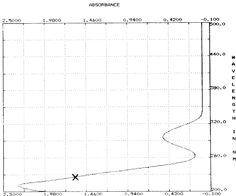
Fig. 3. UV spectrum of flecainide acetate (the cross is at 222 nm).
